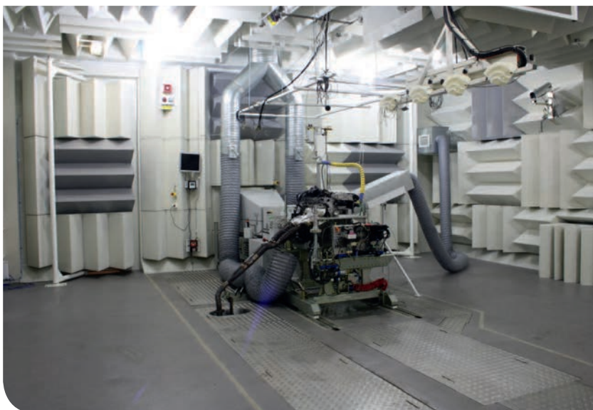
Engine test cell for Volvo
