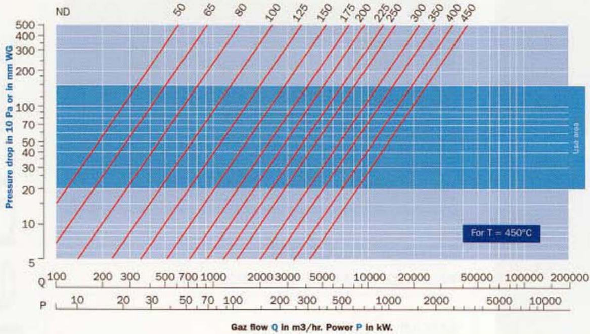
Silencer nominal diameter choice
